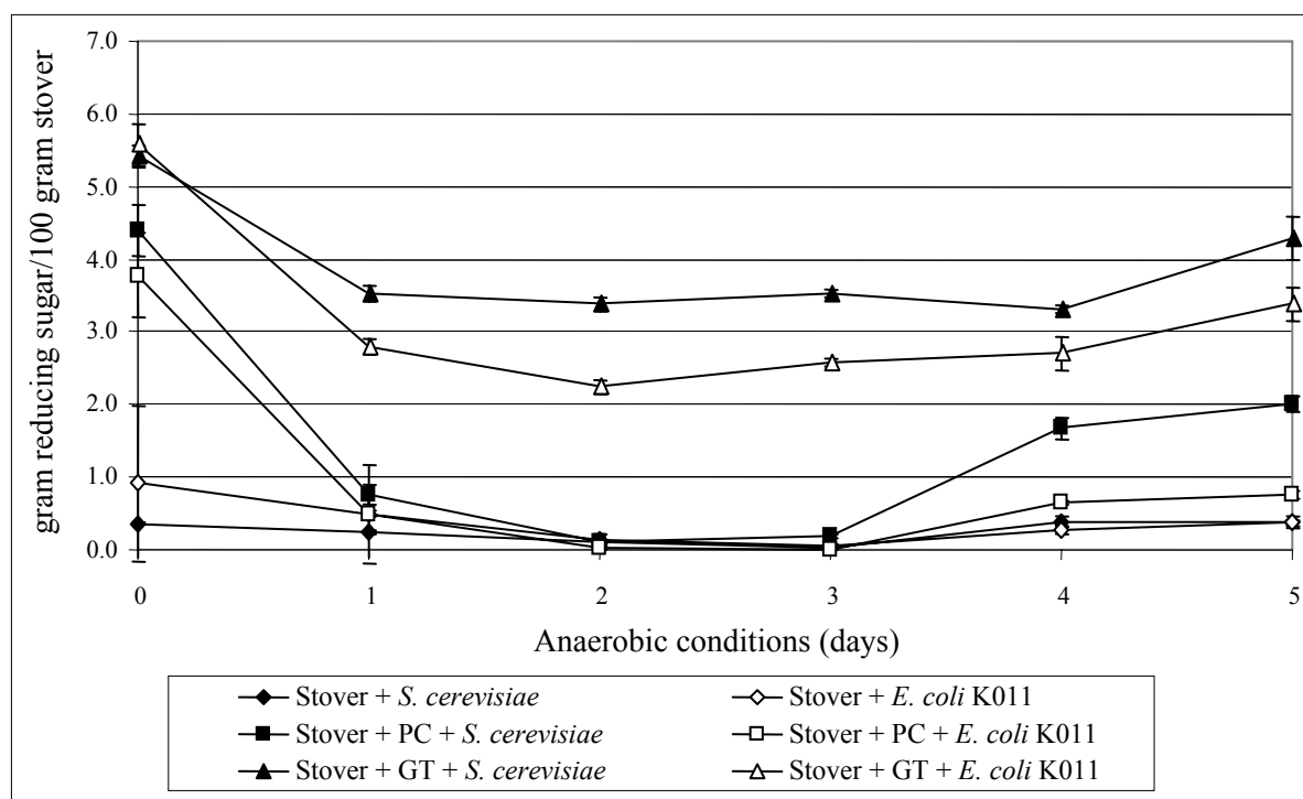
Figure 3. Time course of reducing sugar production, as determined via the Somogyi-Nelson method. The data points represent the averages of three independent experiments (n=3). Note: PC – P. chrysosporium , GT – G. trabeum . Time zero is after 4 days of solid state fermentation with a specific fungus ( P. chrysosporium or G. trabeum ).
