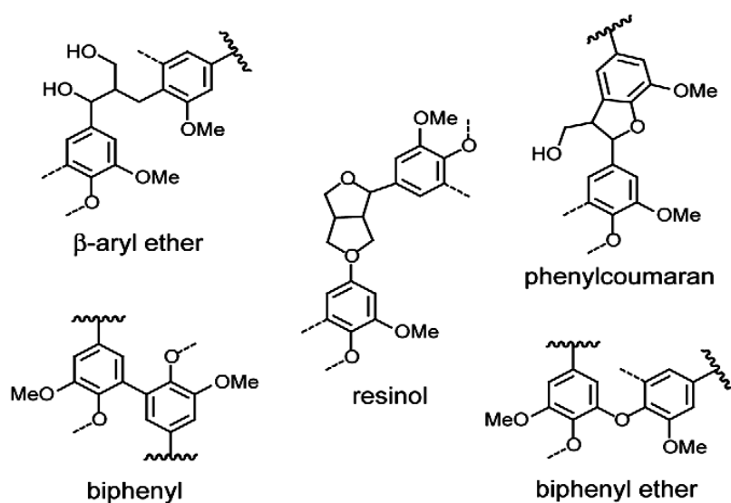
Figure 14. Lignin units crosslinks (Chang, 2007).
