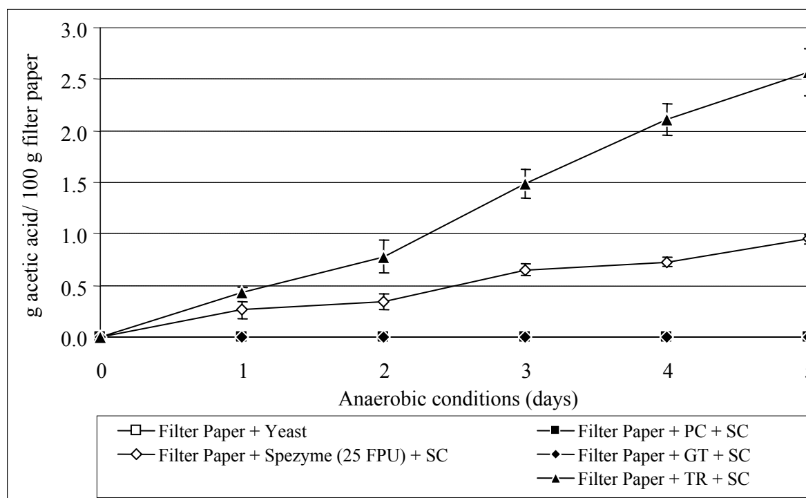
Figure 7. Time course of acetic acid production. The data points represent the averages of three independent experiments ( n=3 ). Note: PC – P. chrysosporium , TR – T. reesei , GT – G. trabeum , SC – S. cerevisia . Time zero is after 4 days of solid state fermentation with a specific fungus ( P. chrysosporium , G. trabeum or T. reesei ).
